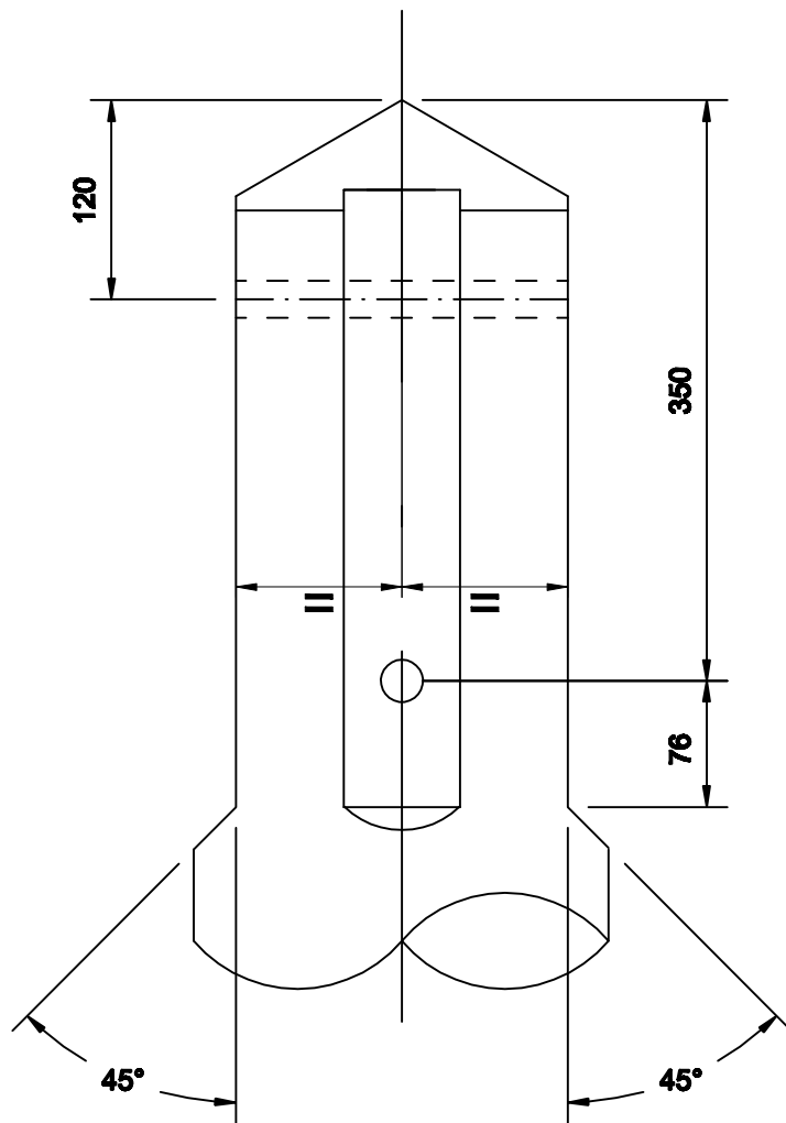
SIDE ELEVATION ON VIEW 'A' & 'B'
