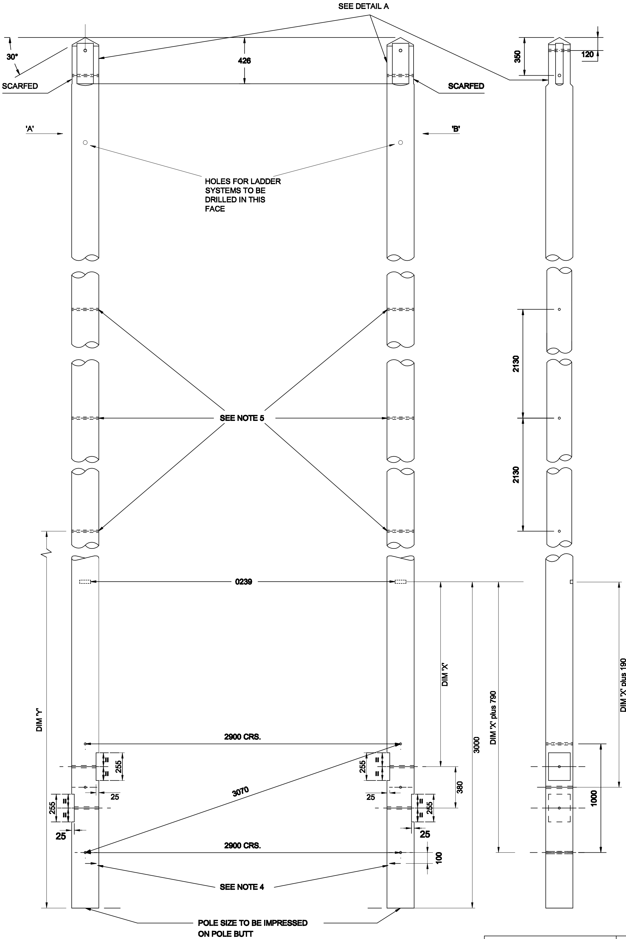
SIDE ELEVATION ON VIEW 'A' & 'B'
